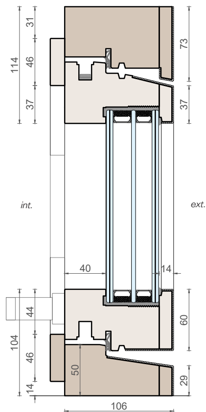
Vertical section
