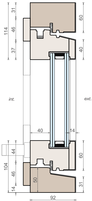
Vertical section
