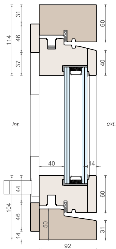
Vertical section
