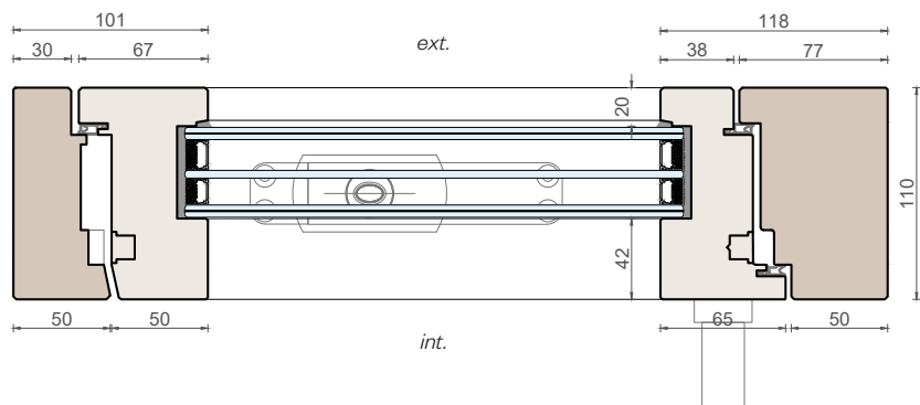
Horizontal section
