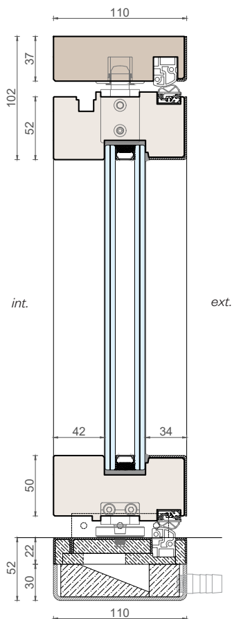
Vertical section
