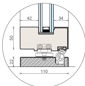
Floor-mounted threshold
