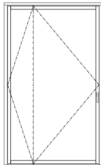
Elevation view
