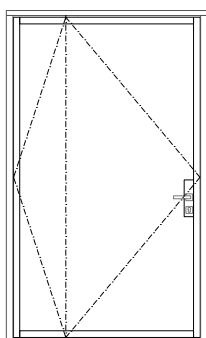
Elevation view
