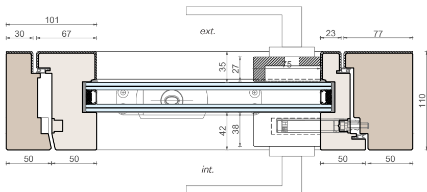
Horizontal section
