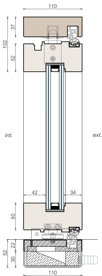
Vertical section
