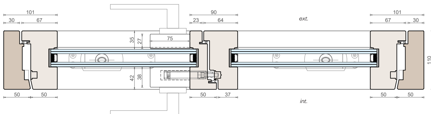
Horizontal section
