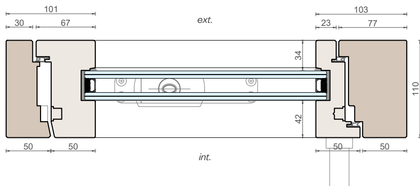
Horizontal section
