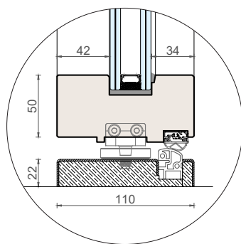
Floor-mounted threshold
