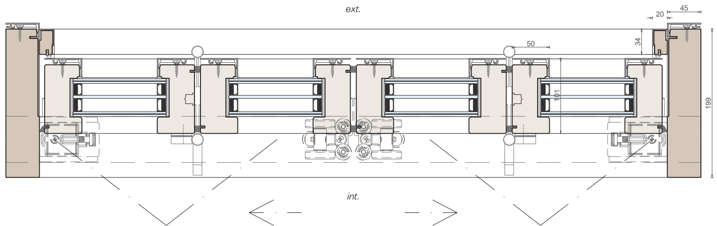
Horizontal section
