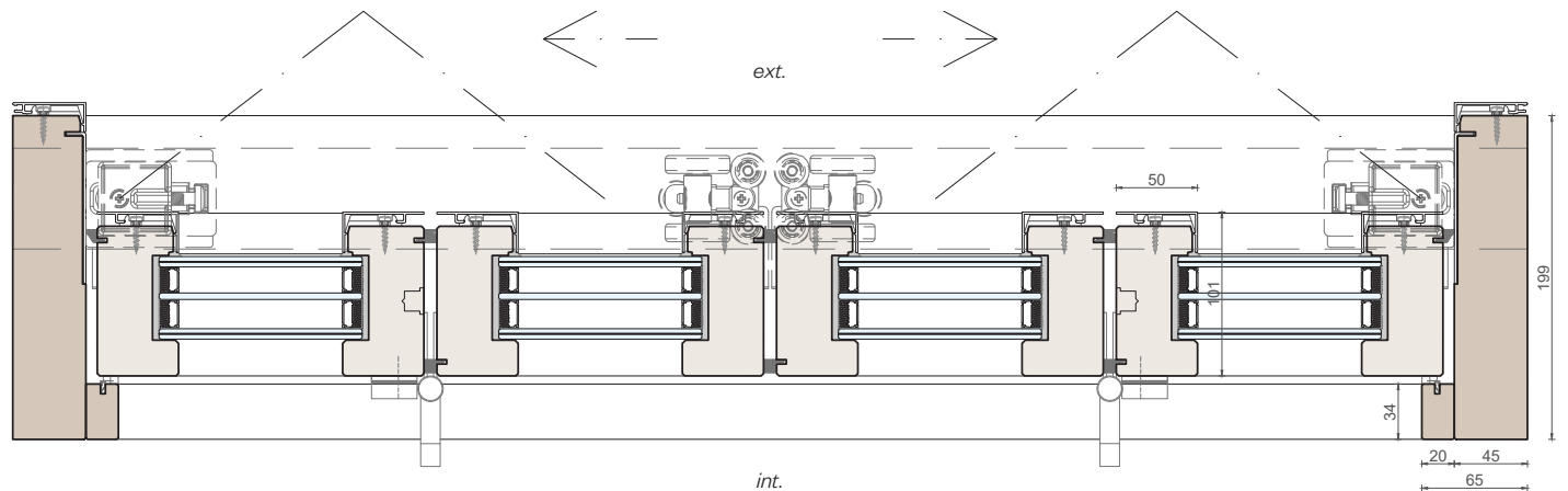
Vertical section
