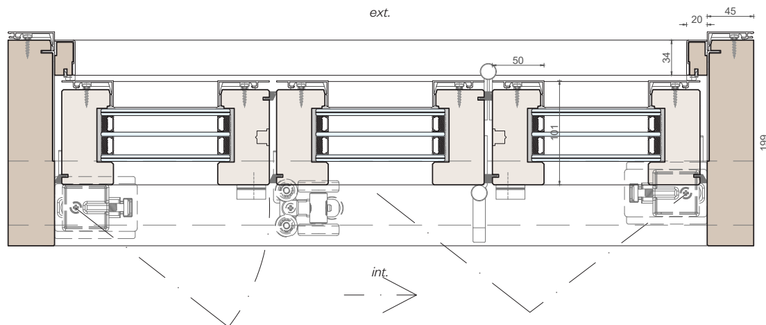
Horizontal section
