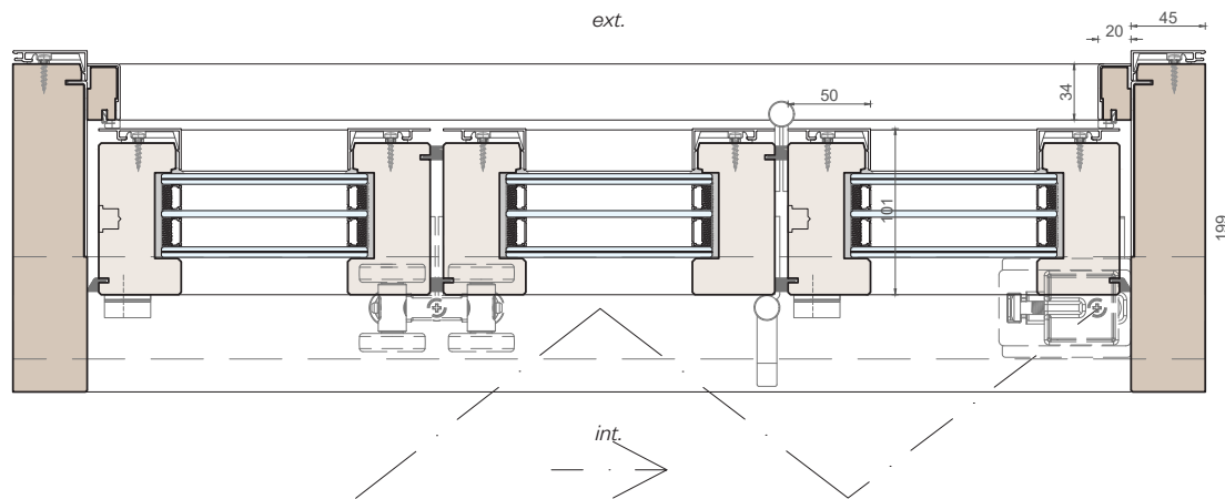
Horizontal section
