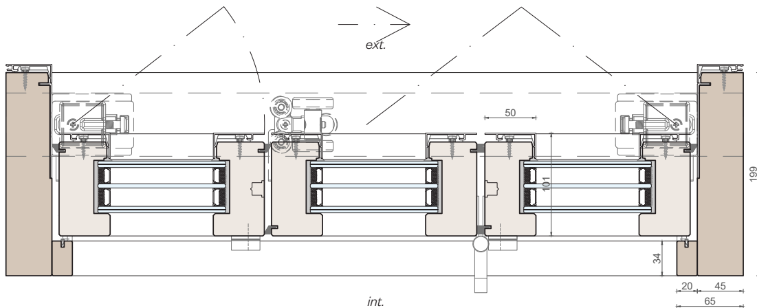
Vertical section
