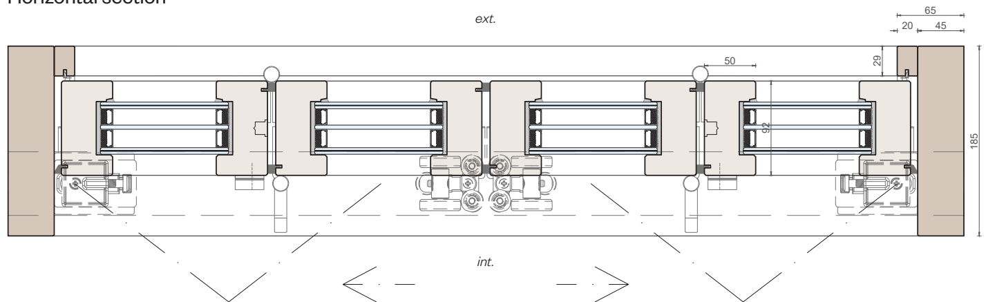
Horizontal section
