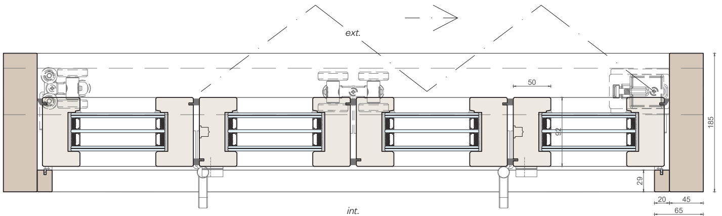
Vertical section
