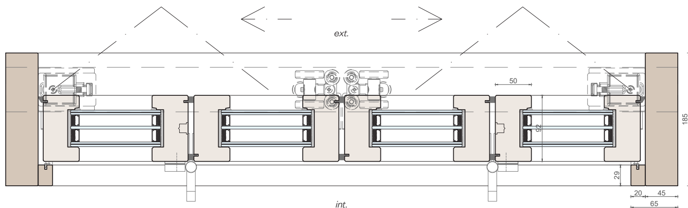
Vertical section
