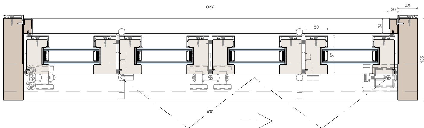
Horizontal section
