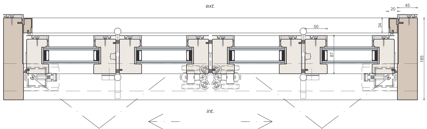
Horizontal section
