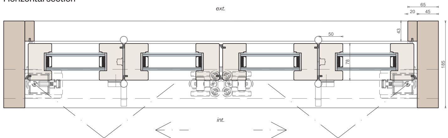
Horizontal section
