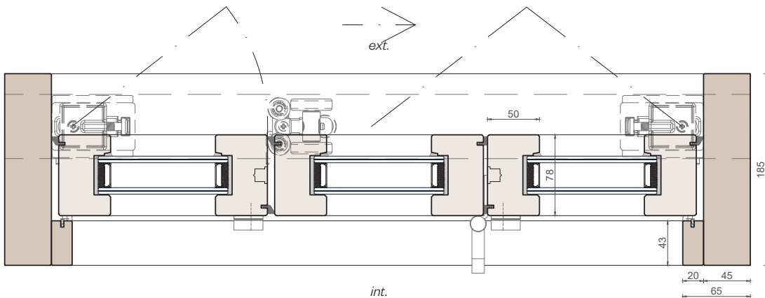
Vertical section
