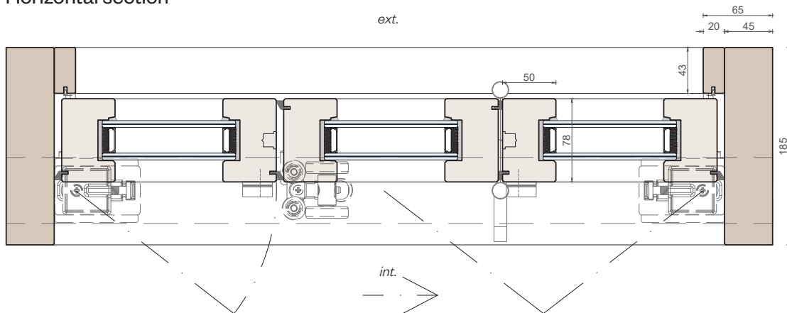
Horizontal section
