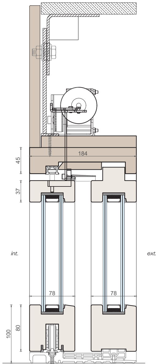
Vertical section
