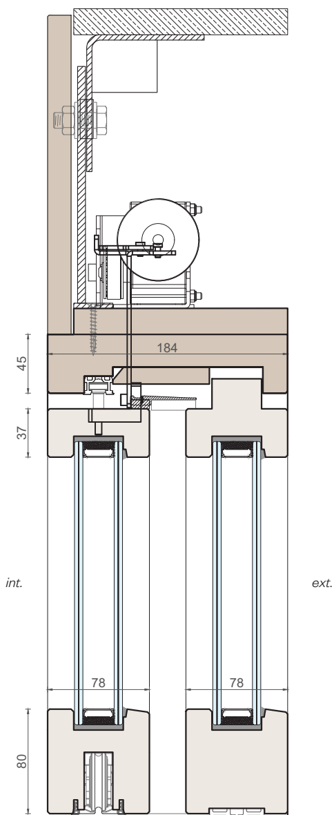
Vertical section
