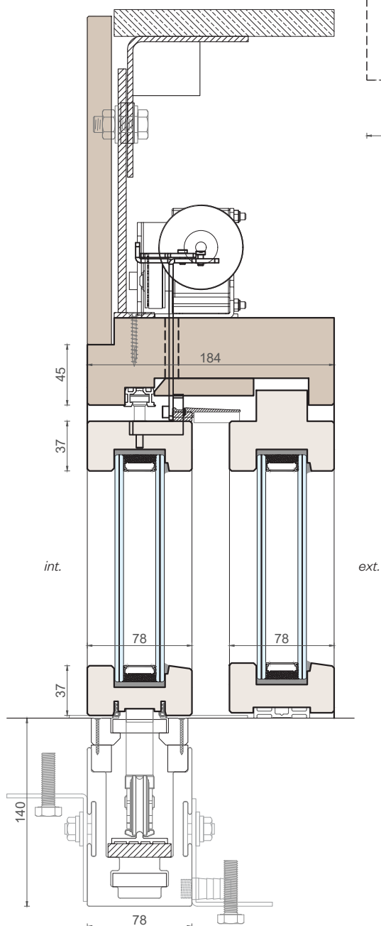
Vertical section
