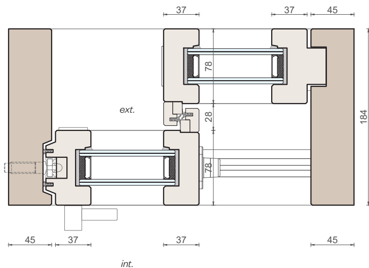
Horizontal section
