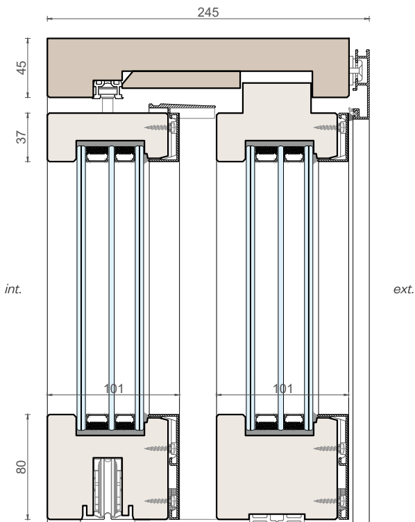
Vertical section
