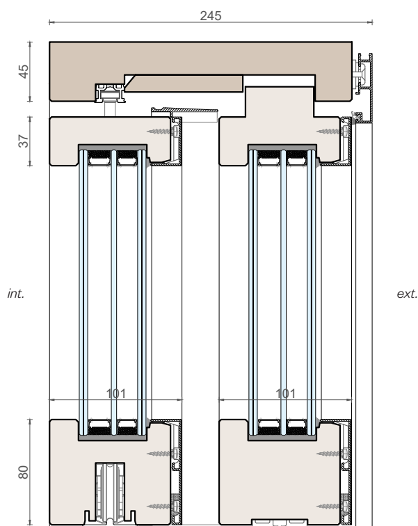
Vertical section
