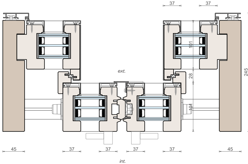
Horizontal section
