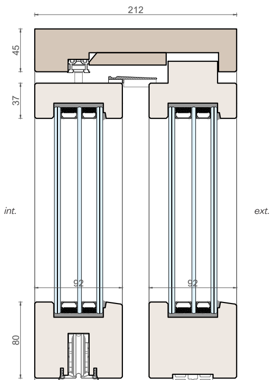
Vertical section
