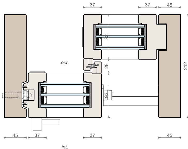
Vertical section
