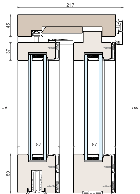
Vertical section
