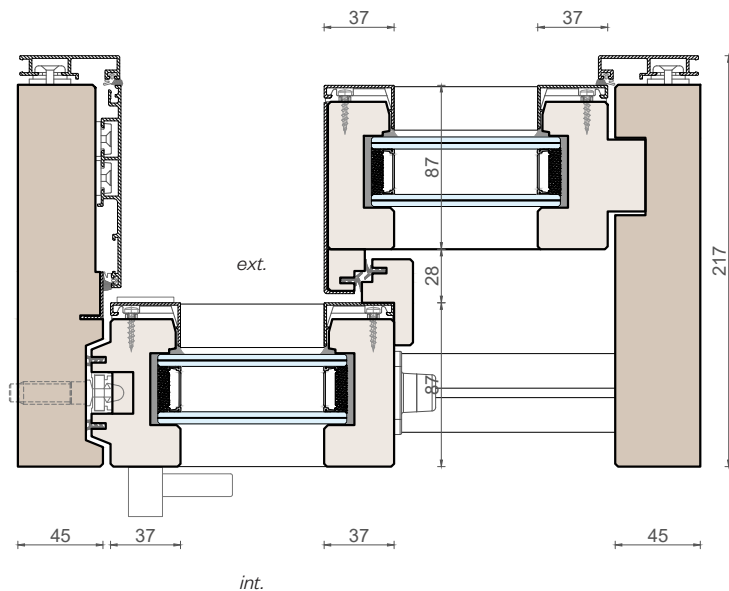
Horizontal section
