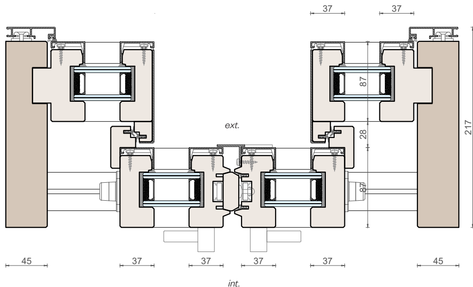
Horizontal section
