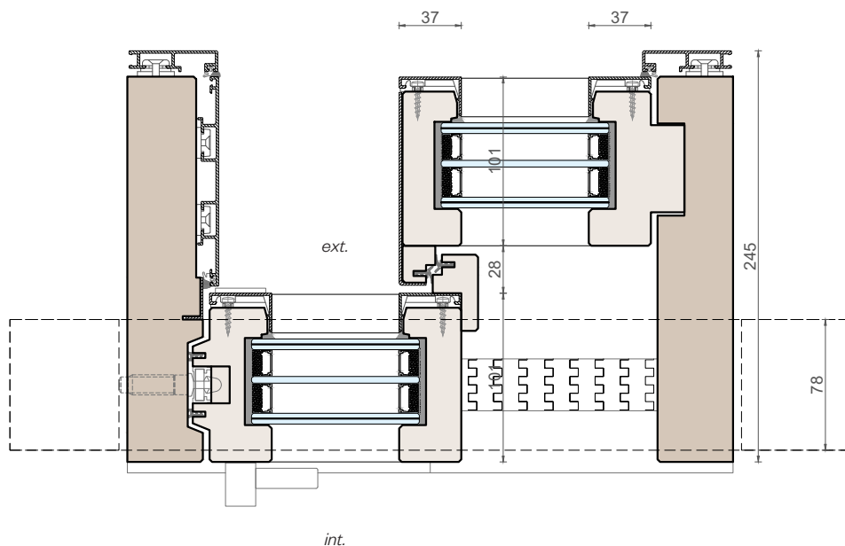
Vertical section
