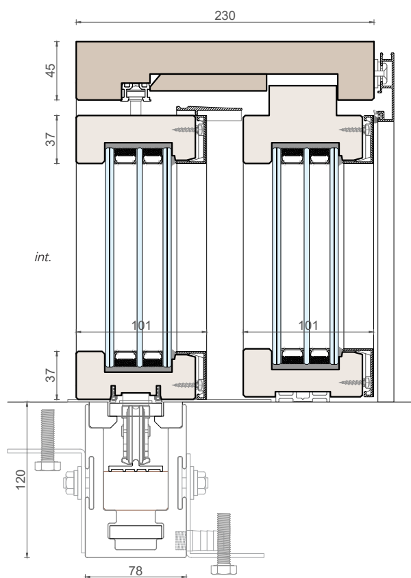
Vertical section
