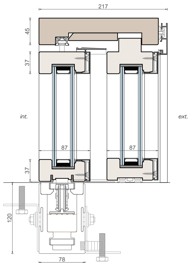
Vertical section
