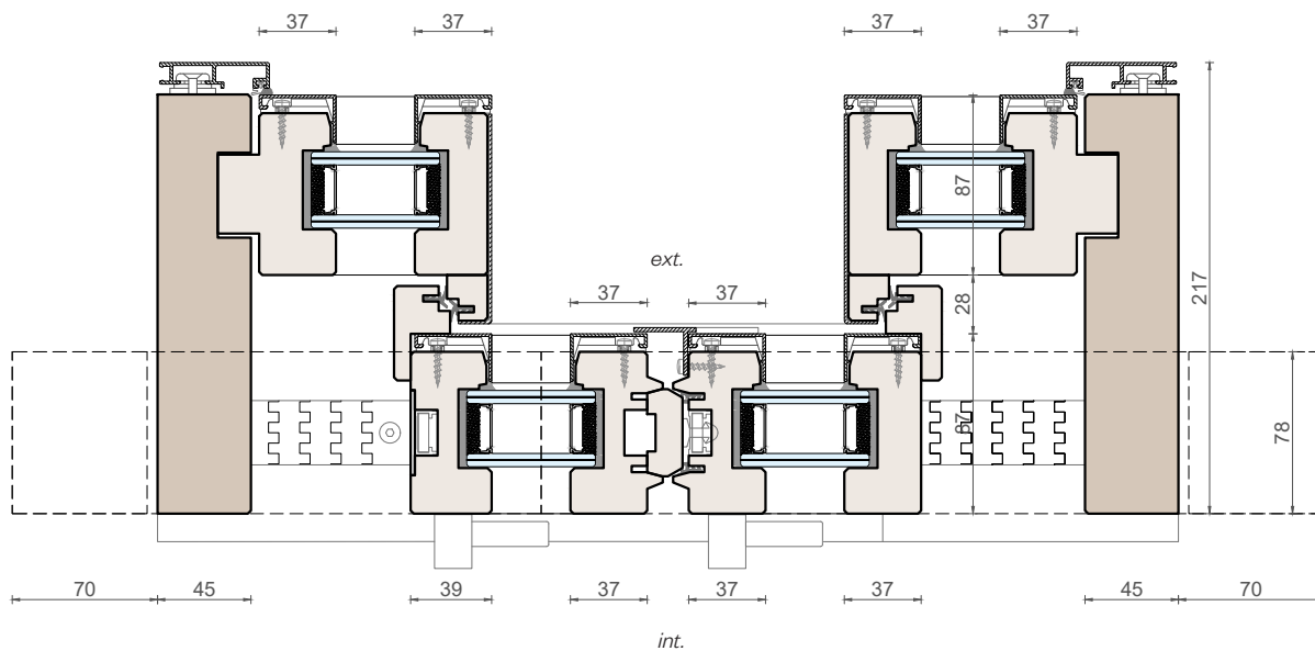
Vertical section
