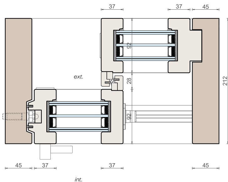
Vertical section
