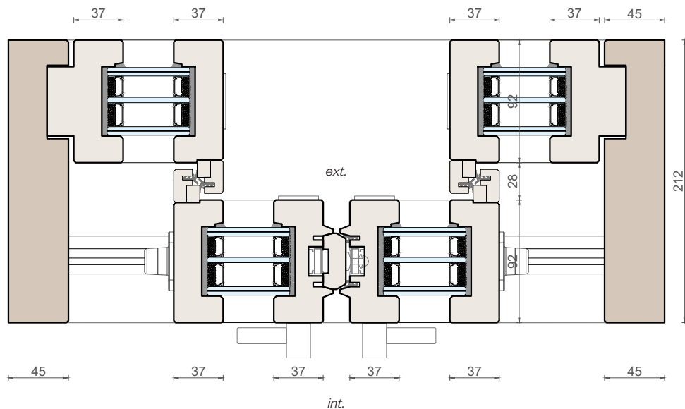
Vertical section
