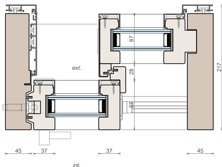
Horizontal section
