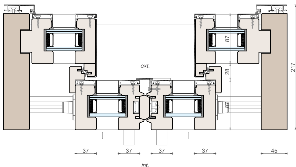
Horizontal section
