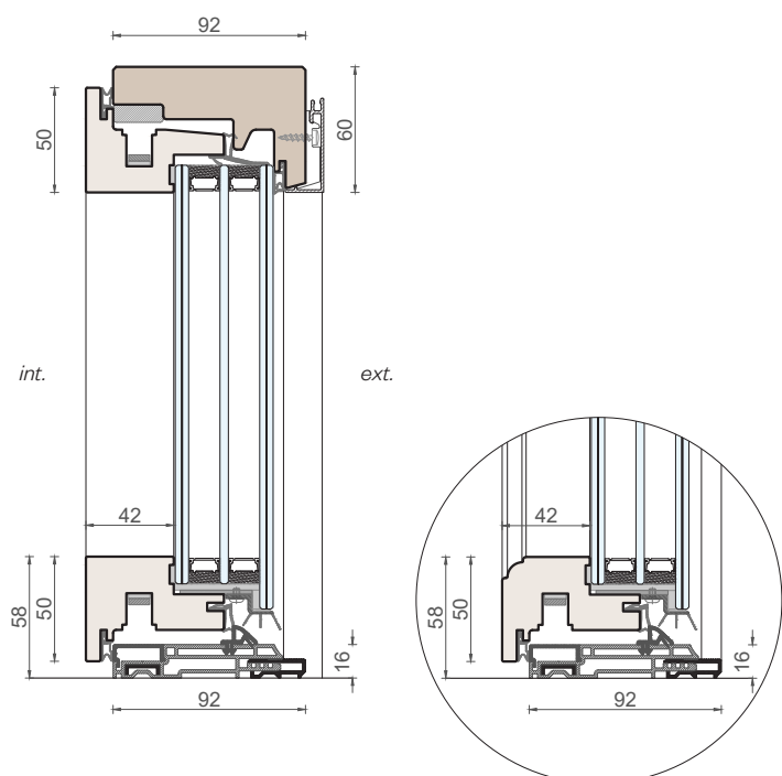
Vertical section
