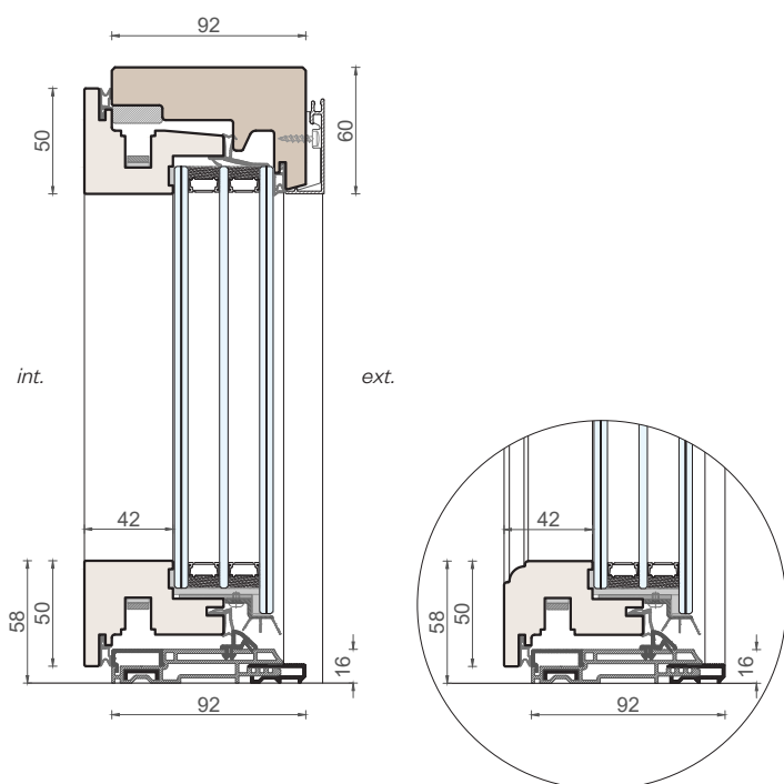
Vertical section
